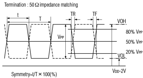
Figure 5) Output Waveform (1)
