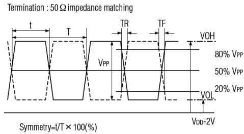
Figure 6) Output Waveform (2)
