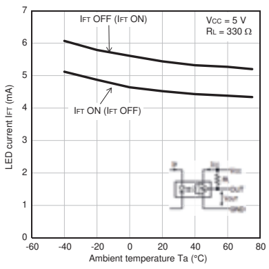
Fig 4. LED Current vs. Ambient Temperature Characteristics (Typical)
