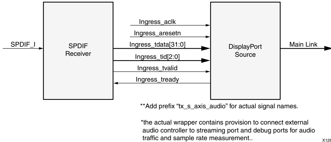
Figure 2: Audio Data Interface of DisplayPort Source System
