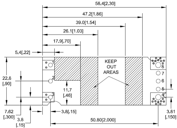
SMT Recommend Pad Layout (Component Side View)
