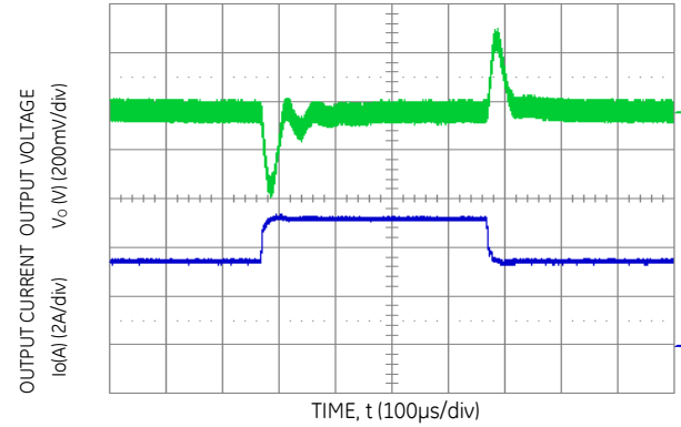
Figure 4. Transient Response to 1.0A/ \mu s Dynamic Load Change from 50% to 75% to 50% of full load.
