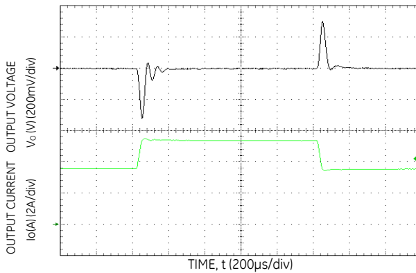
Figure 3. Transient Response to 0.1A/ \mu s Dynamic Load Change from 50% to 75% to 50% of full load.
