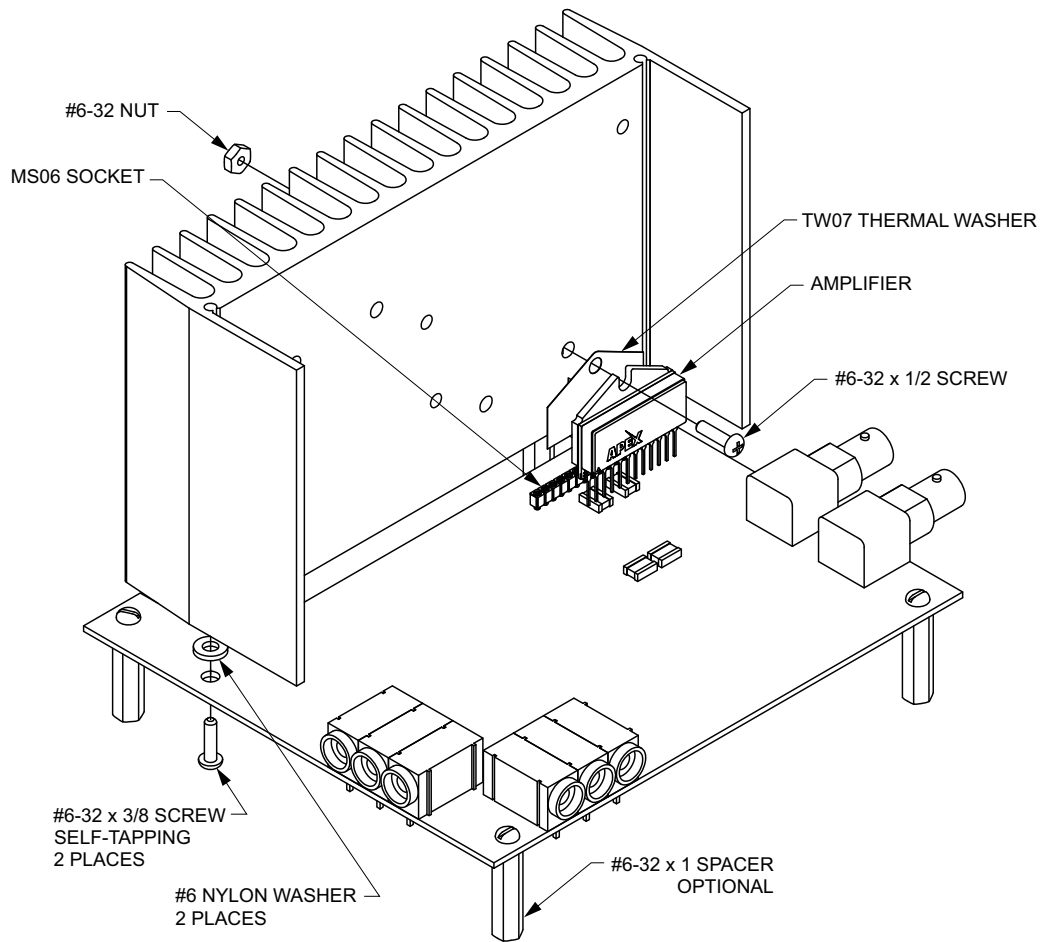
Figure 3: Assembly Diagram
