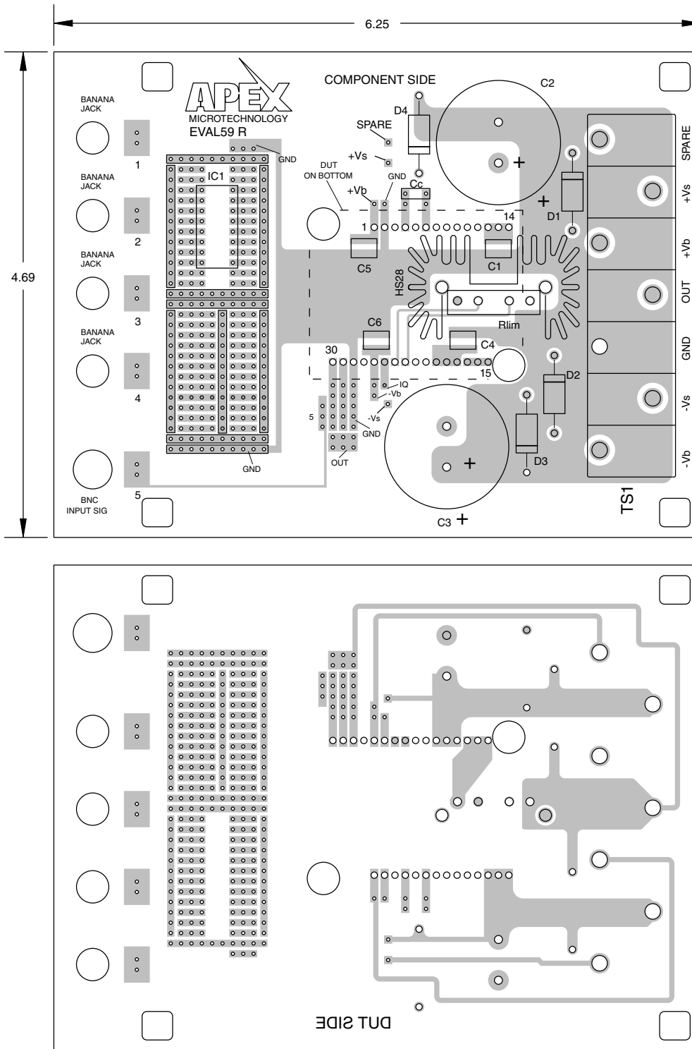
Figure 2: PCB
