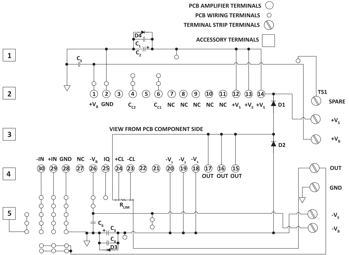
Figure 1: External Connections
