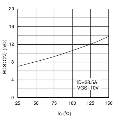
RDS(ON)-Tc characteristics (typical)
