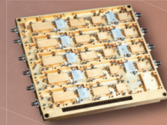
Multi-Channel Downconverter
