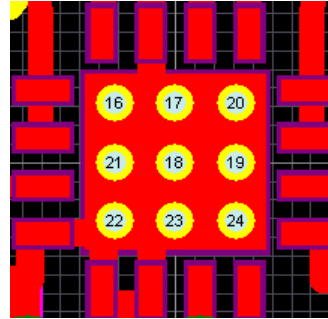
TOP (16 Ld QFN)
