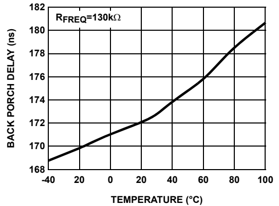
FIGURE 30. BACK PORCH DELAY vs TEMPERATURE - FSEL = 0
