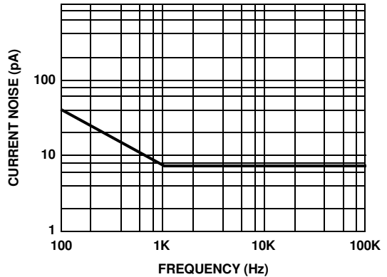
FIGURE 20. CURRENT NOISE
