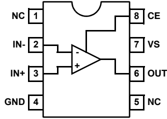
EL5146 (8 LD SO, PDIP) TOP VIEW
