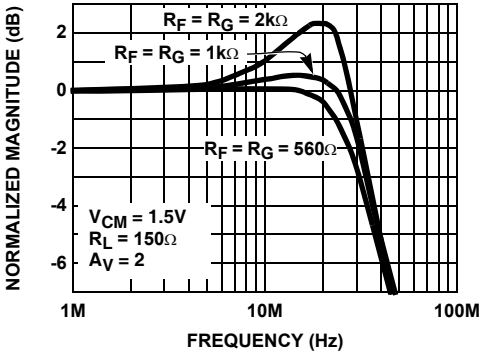
FIGURE 9. FREQUENCY RESPONSE FOR VARIOUS R_F AND R_G
