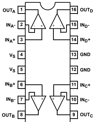
EL5444 (16 LD QSOP) TOP VIEW
