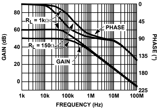
FIGURE 11. OPEN LOOP GAIN AND PHASE vs FREQUENCY
