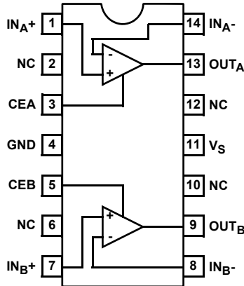
EL5246 (14 LD SOIC, PDIP) TOP VIEW
