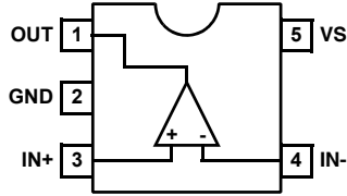
EL5144 (5 LD SOT-23) TOP VIEW
