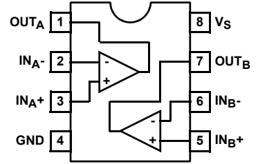
EL5244 (8 LD SOIC, PDIP, MSOP) TOP VIEW
