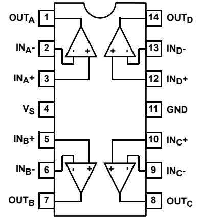
EL5444 (14 LD SOIC, PDIP) TOP VIEW
