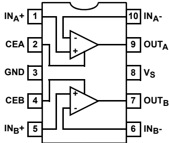
EL5246 (10 LD MSOP) TOP VIEW
