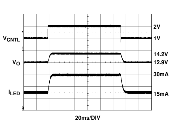
FIGURE 16. TRANSIENT RESPONSE
