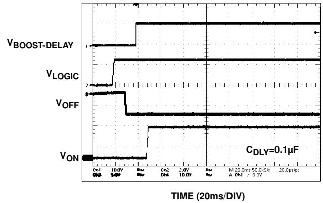
FIGURE 12. EL7520 START-UP SEQUENCE
