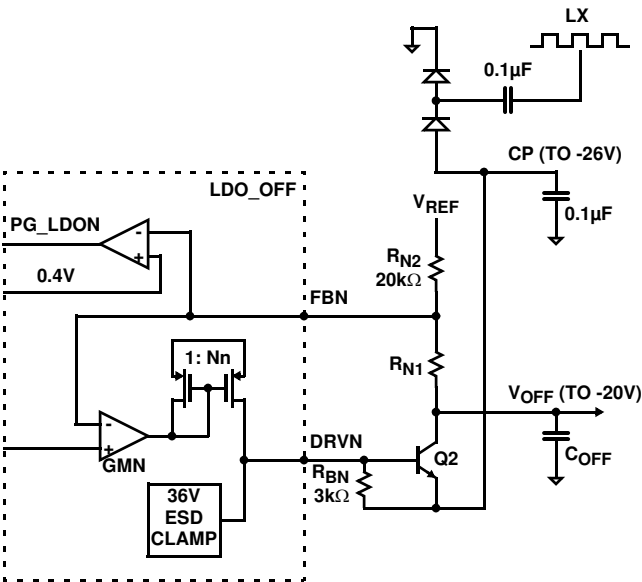
FIGURE 28. V_{OFF} FUNCTIONAL BLOCK DIAGRAM
