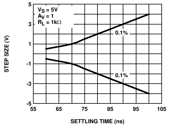
FIGURE 22. SETTLING TIME vs STEP SIZE
