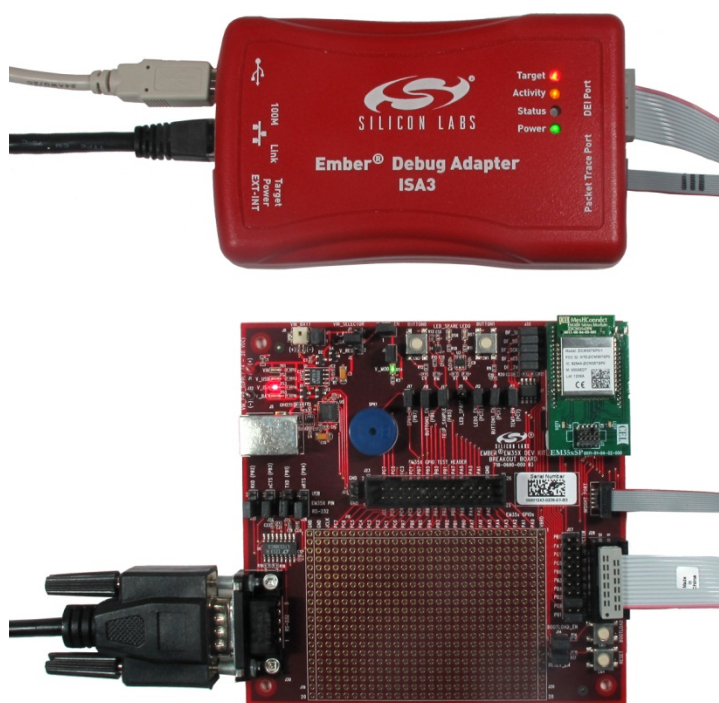
Figure 5.8. Debug Adapter (ISA3) Supplying Power; RS-232 Serial Communication
