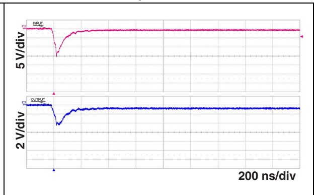
Figure 8. ESD response to IEC 61000-4-2 (-15 kV air discharge) applied to external pin
