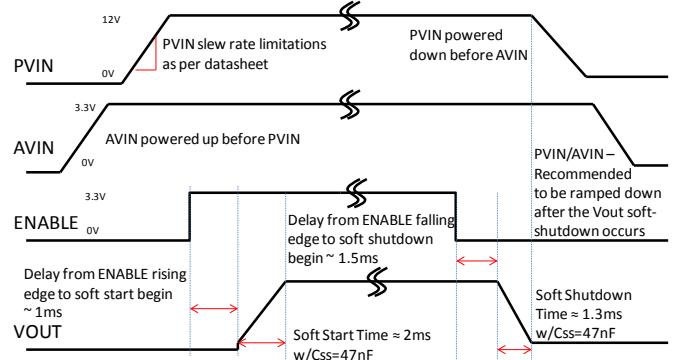
Figure 8: Dual Supply Startup/Shutdown Sequencing
