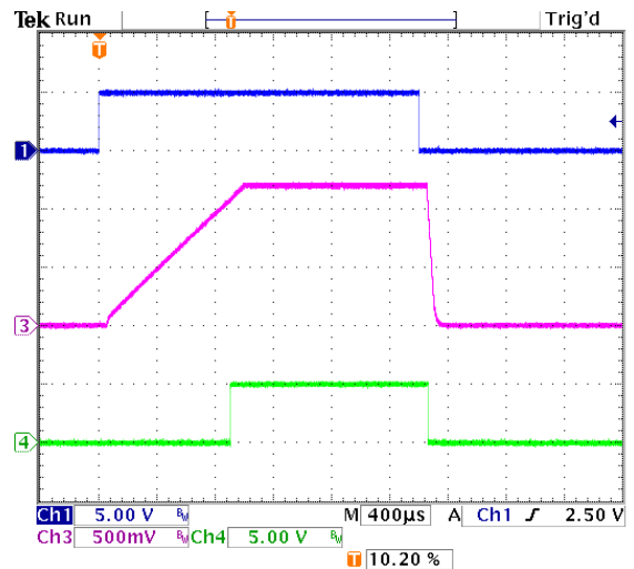
Power Up/Down into 0.4Ω load: V_{IN}/V_{OUT} = 5.0V/1.2V , 15nF soft-start capacitor, Ch.1: ENABLE, Ch.3: V_{OUT} , Ch.4: POK
