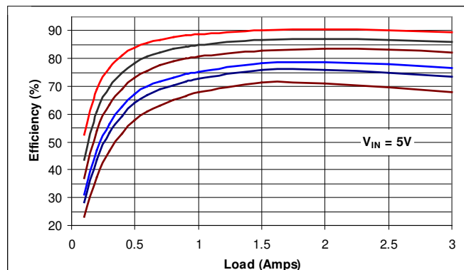
Efficiency V_{IN} = 5.0V
