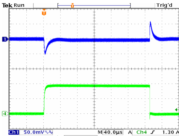
Transient Response: 5V_{IN}/1.2V_{OUT} , 0-9A , 7A/\mu S . C_{OUT} = 5x22\mu F .
