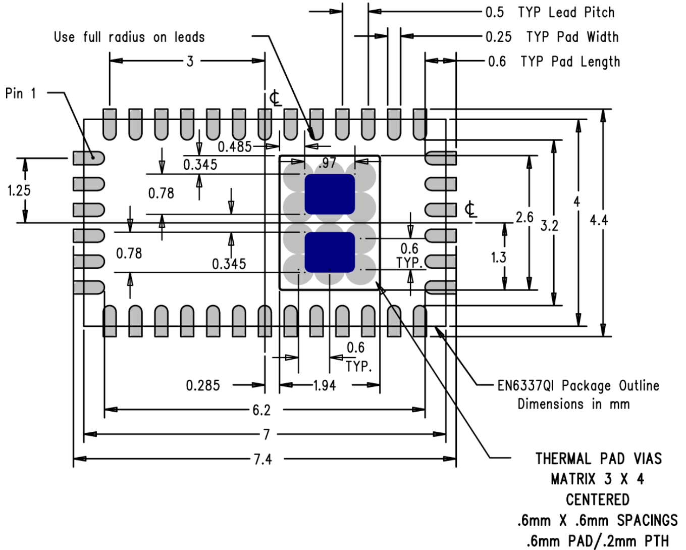
Figure 12: EN6337QI PCB Footprint (Top View)
