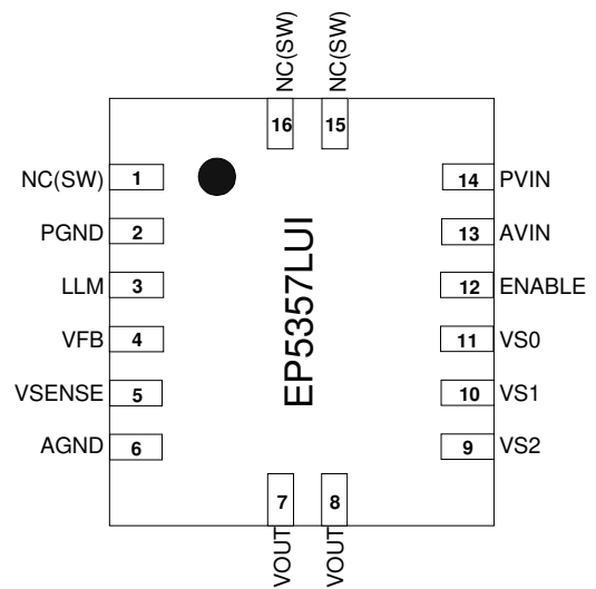
Figure 3: EP5357LUI Pin Out Diagram (Top View)
