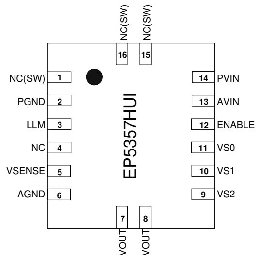
Figure 4: EP5357HUI Pin Out Diagram (Top View)
