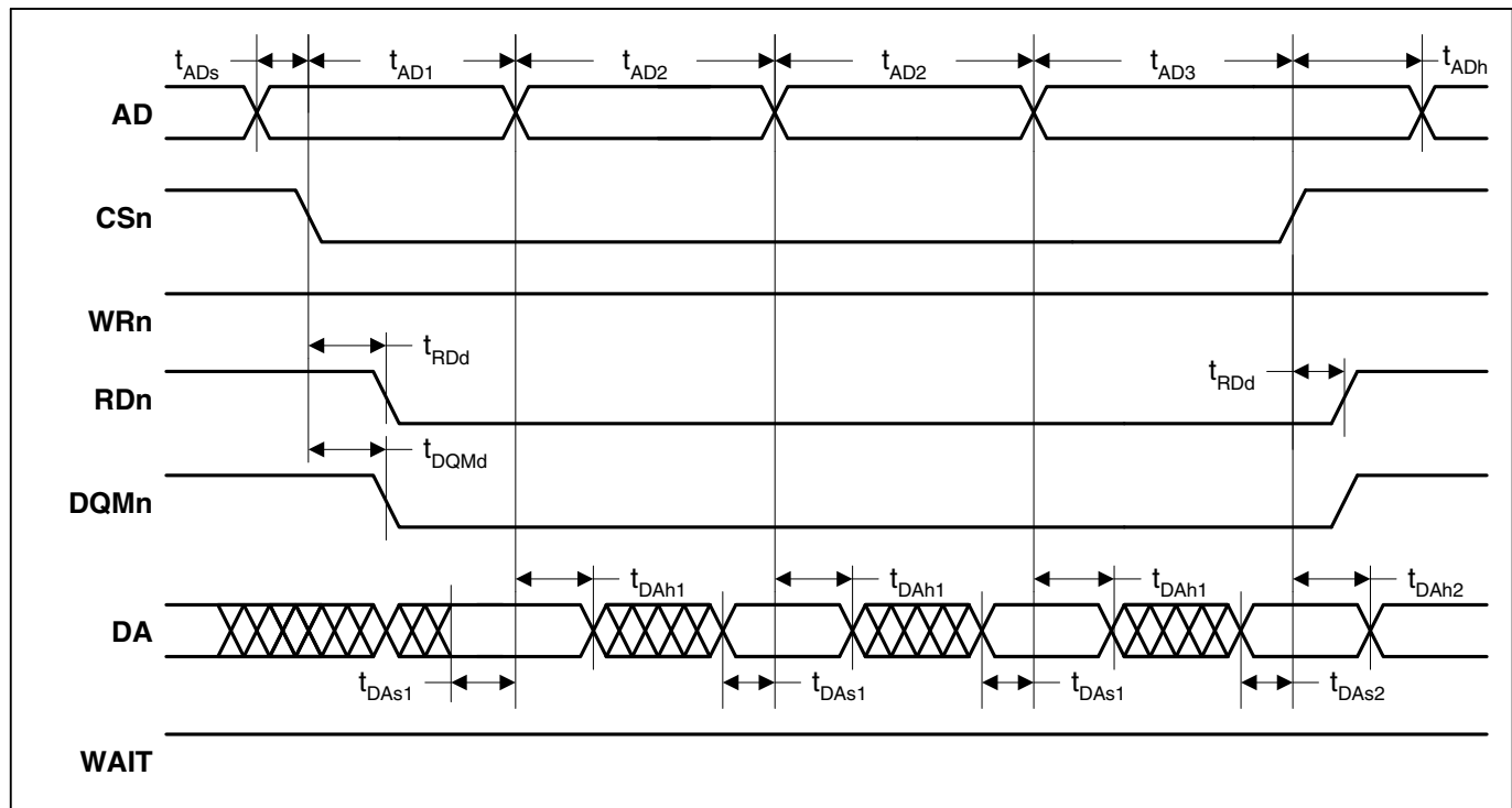
Figure 6. Static Memory Multiple Word Read 8-bit Cycle Timing Measurement
