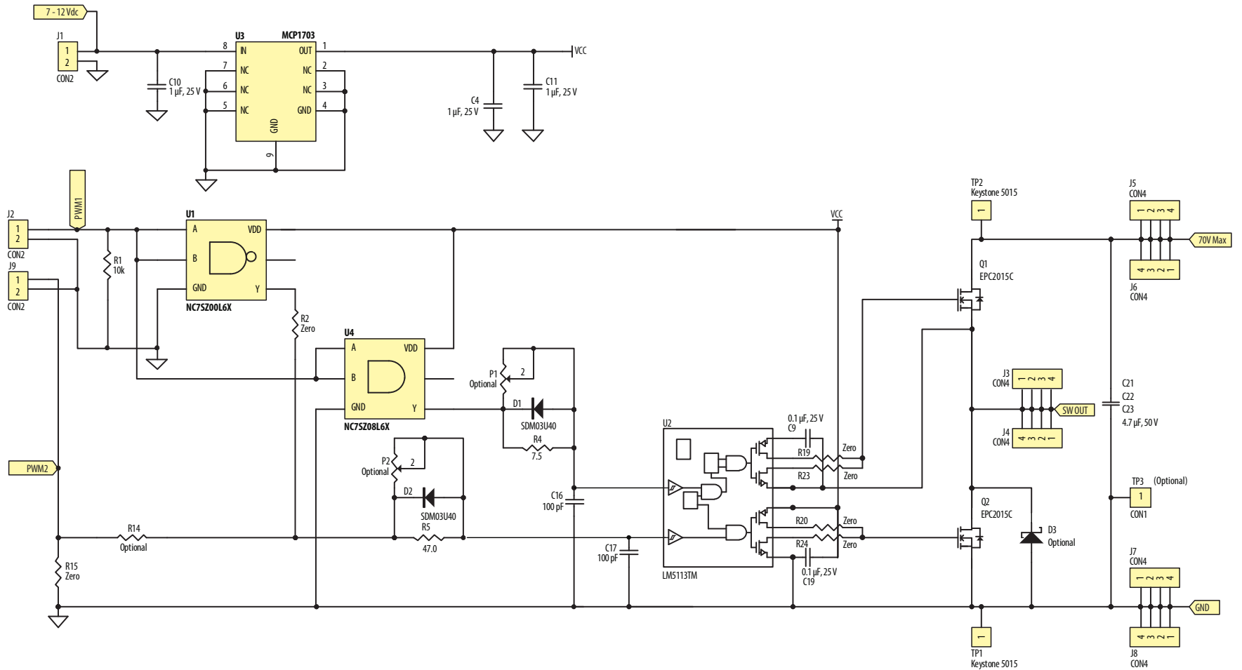
Development Board EPC9001C Schematic Rev 5.0
