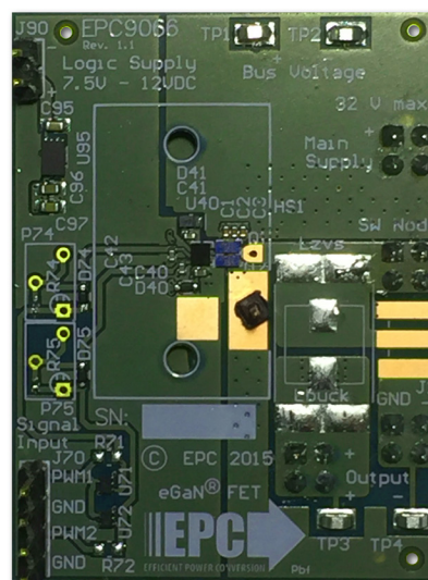
EPC9066 amplifier board photo
