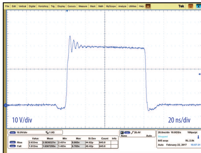
Figure 3: Typical Waveform for V_{IN} = 48 \text{ V} to 1.8 \text{ V}_{OUT} , 20 A (500 kHz) Buck Converter.
