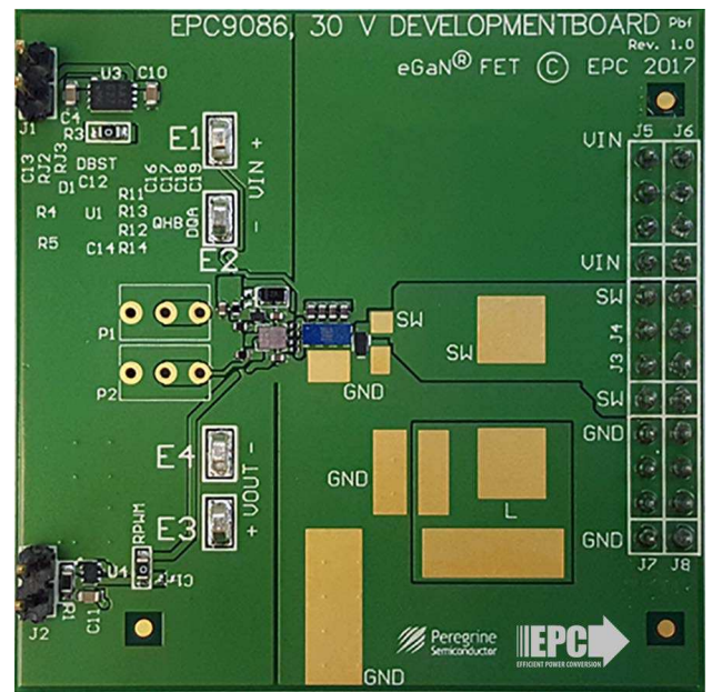
EPC9086 board.
