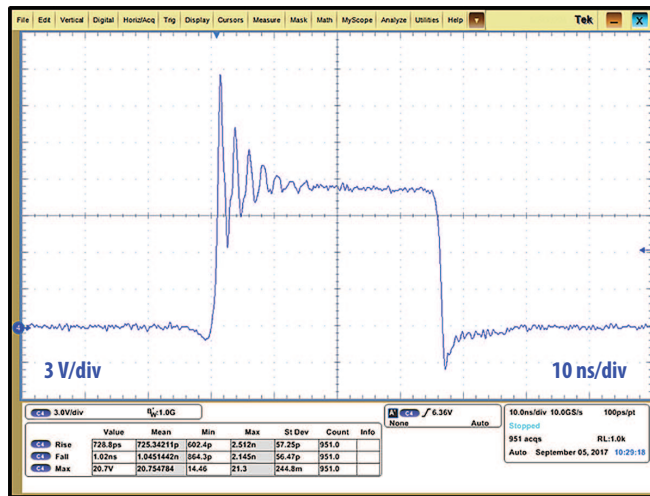
Figure 3: Typical waveform for V_{IN} = 12\text{ V} to 1.8\text{ V}_{OUT} , 10 A (5 MHz) buck converter.
