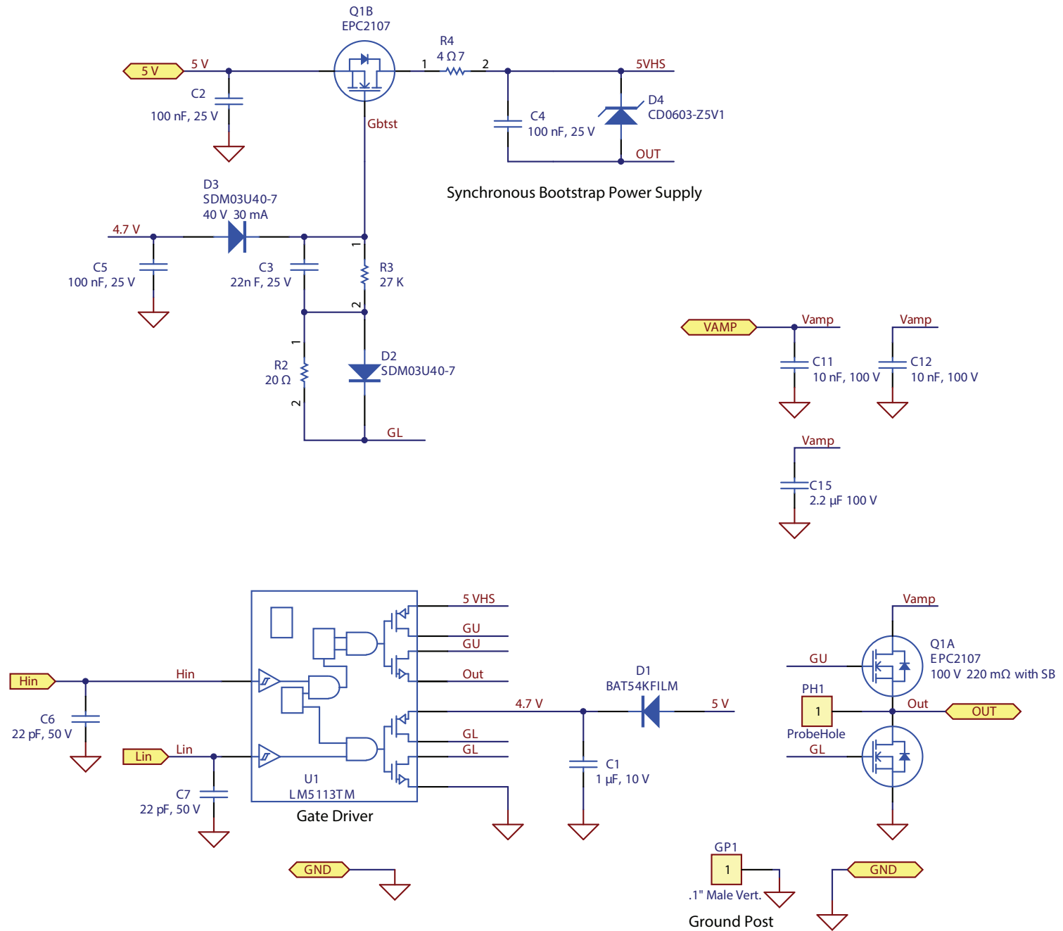
Figure 14: EPC9511 - Gate driver and power devices schematic
