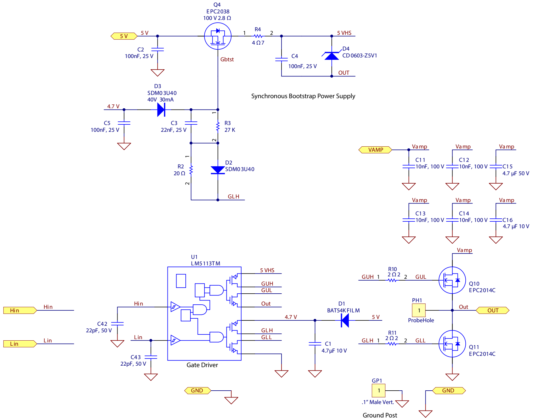
Figure 5: EPC9506 Source Board Amplifier Schematic
