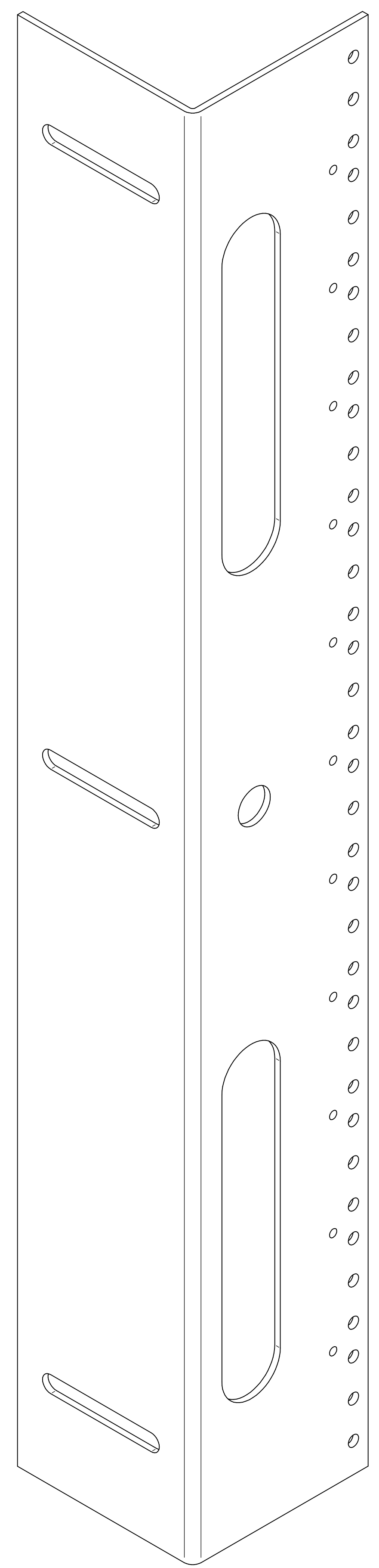
ISOMETRIC VIEW
