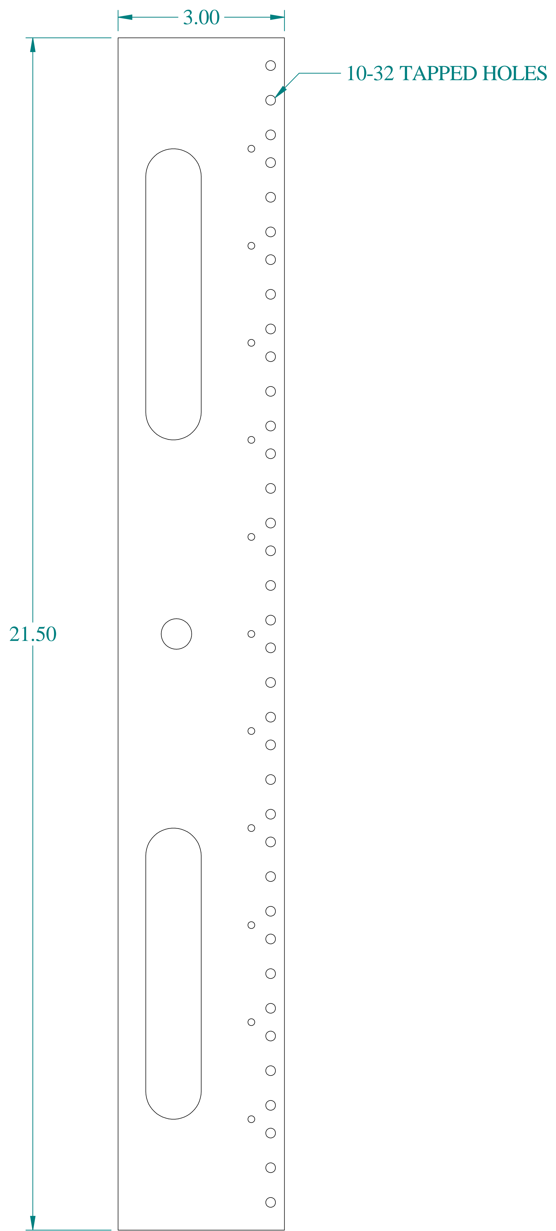
FRONT VIEW
