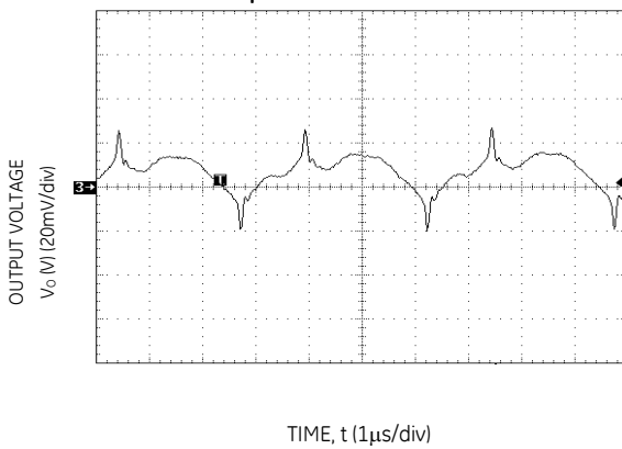
Figure 20. Typical Output Ripple and Noise (Vin =48Vdc, Io = 23A).
