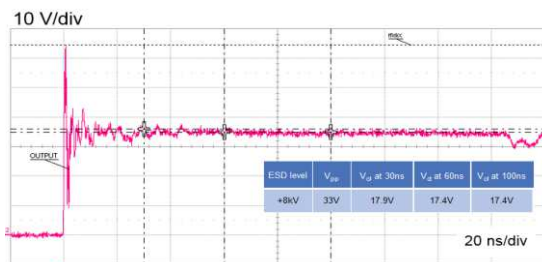
Figure 7: ESD response to IEC 61000-4-2 (+8kV contact discharge)
