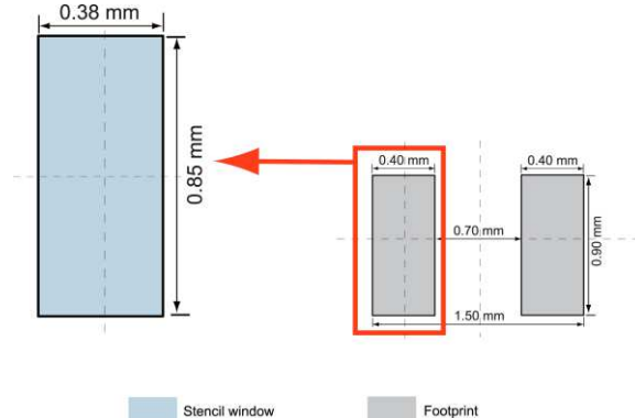
Figure 16: Alternative stencil window position
