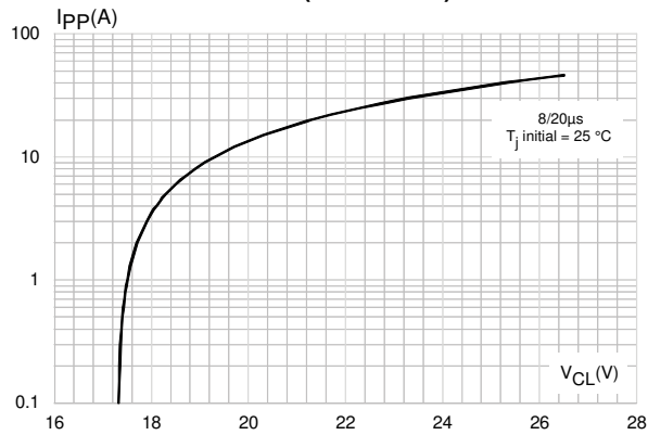
Figure 5: Clamping voltage versus peak pulse current (max. value)
