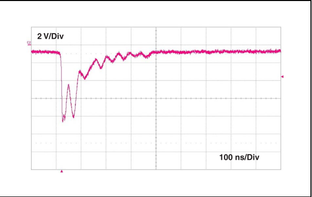
Figure 8. ESD response to IEC 61000-4-2 (-30 kV air discharge)
