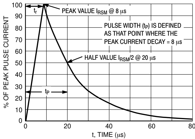
Figure 8. 8 X 20 \mu s Pulse Waveform
