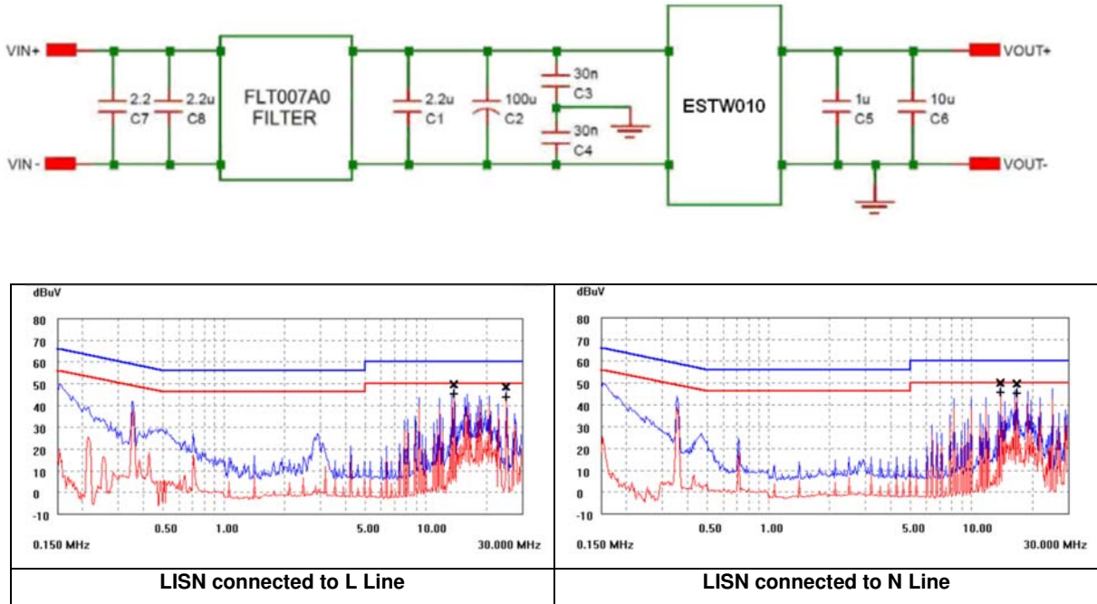
Figure 26. EMC Considerations
