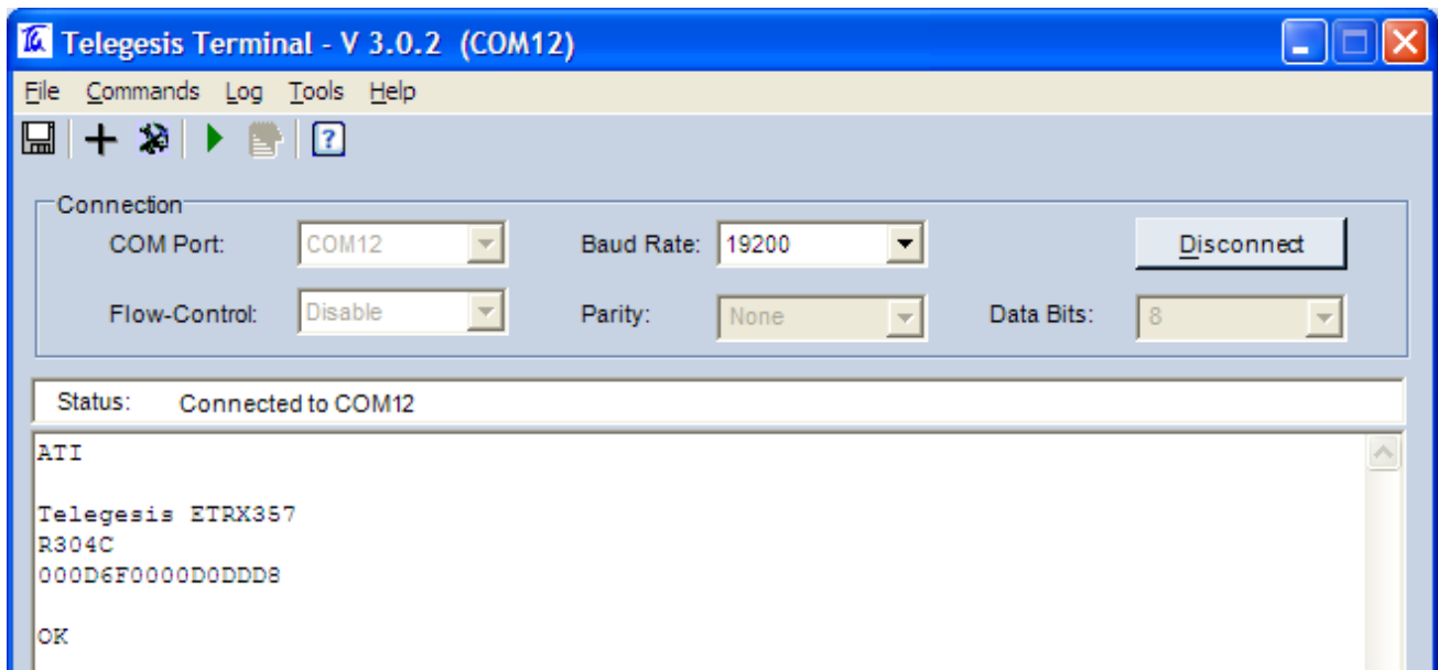
Figure 3. Telegesis Terminal
