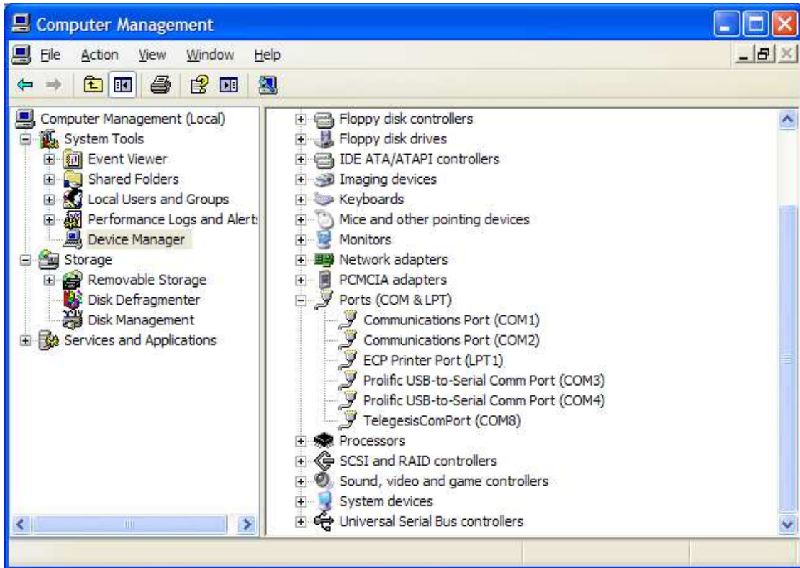
Figure 2. Device Manager
