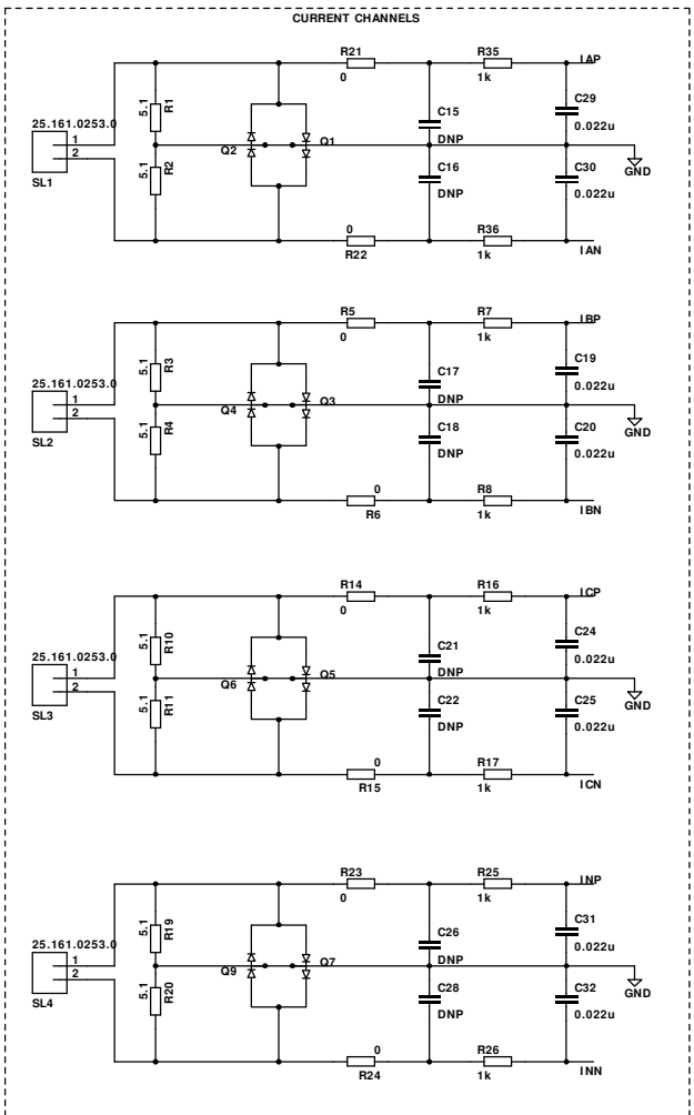
Figure 5. EV-ADE9000SHIELDZ Schematic Sheet 1
