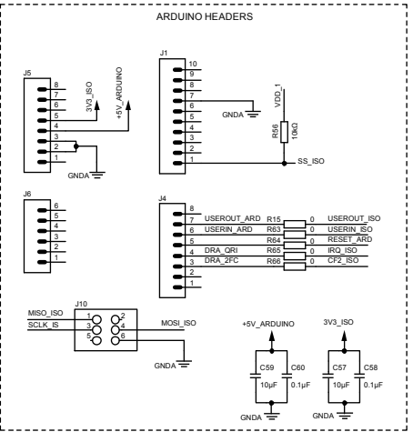
Figure 4. EV-ADE9153ASHIELDZ Schematic
