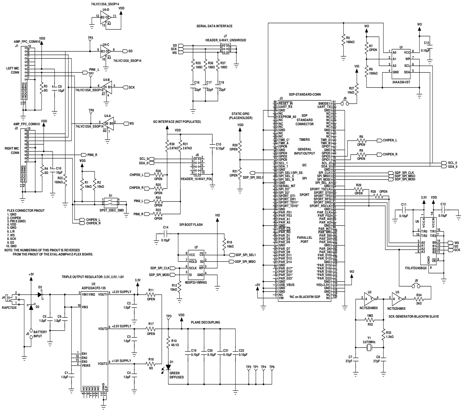
Figure 9. Schematic of the Evaluation Board
