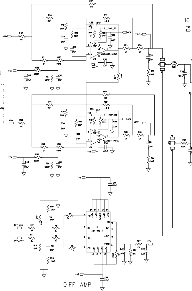
Figure 27. ADC Evaluation Board, ADC Drivers and ADC
