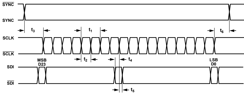
Figure 6. LVDS Timing
