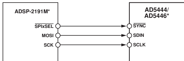
Figure 45. ADSP-2191M SPI to AD5444/AD5446 Interface
