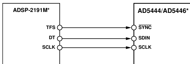
Figure 46. ADSP-2191M to AD5444/AD5446 Interface
