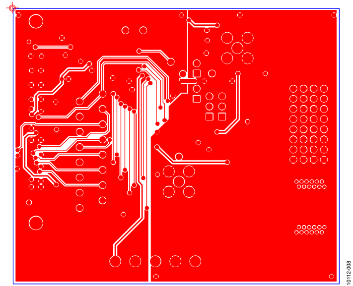
Figure 8. Component Side
