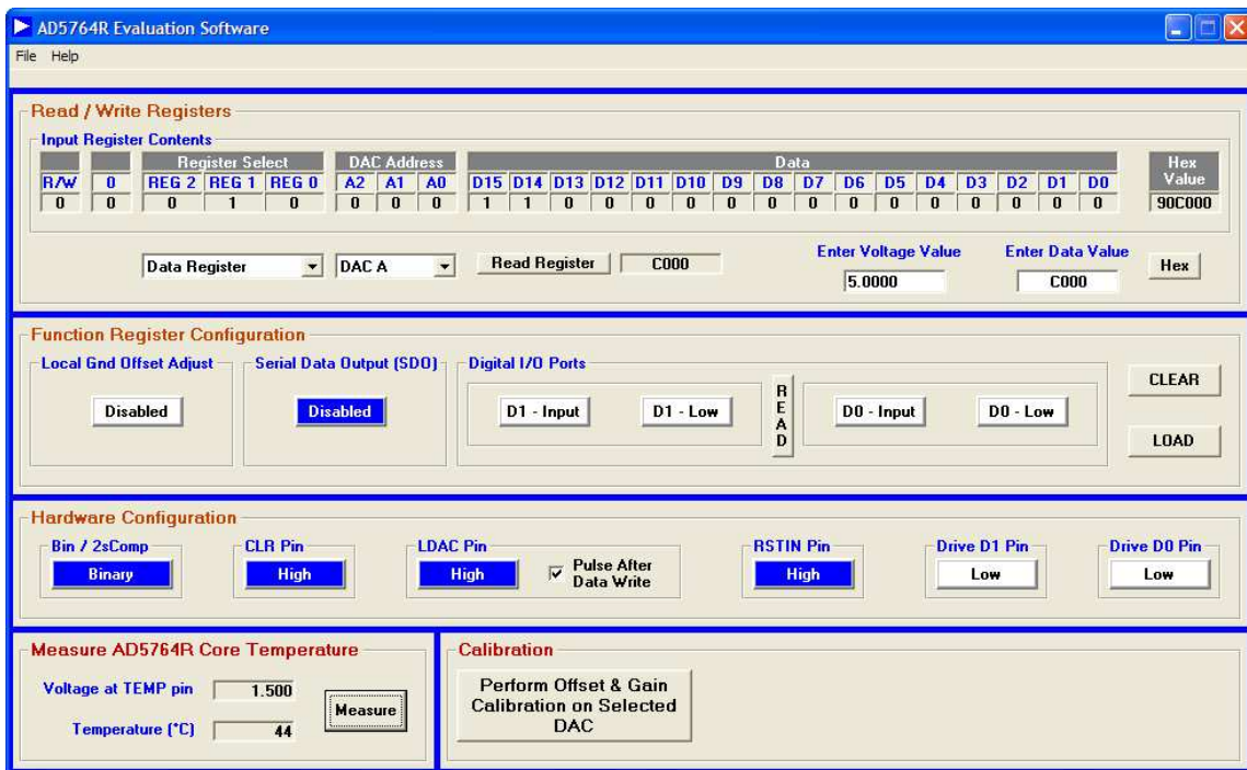
Figure 2. Main Window
