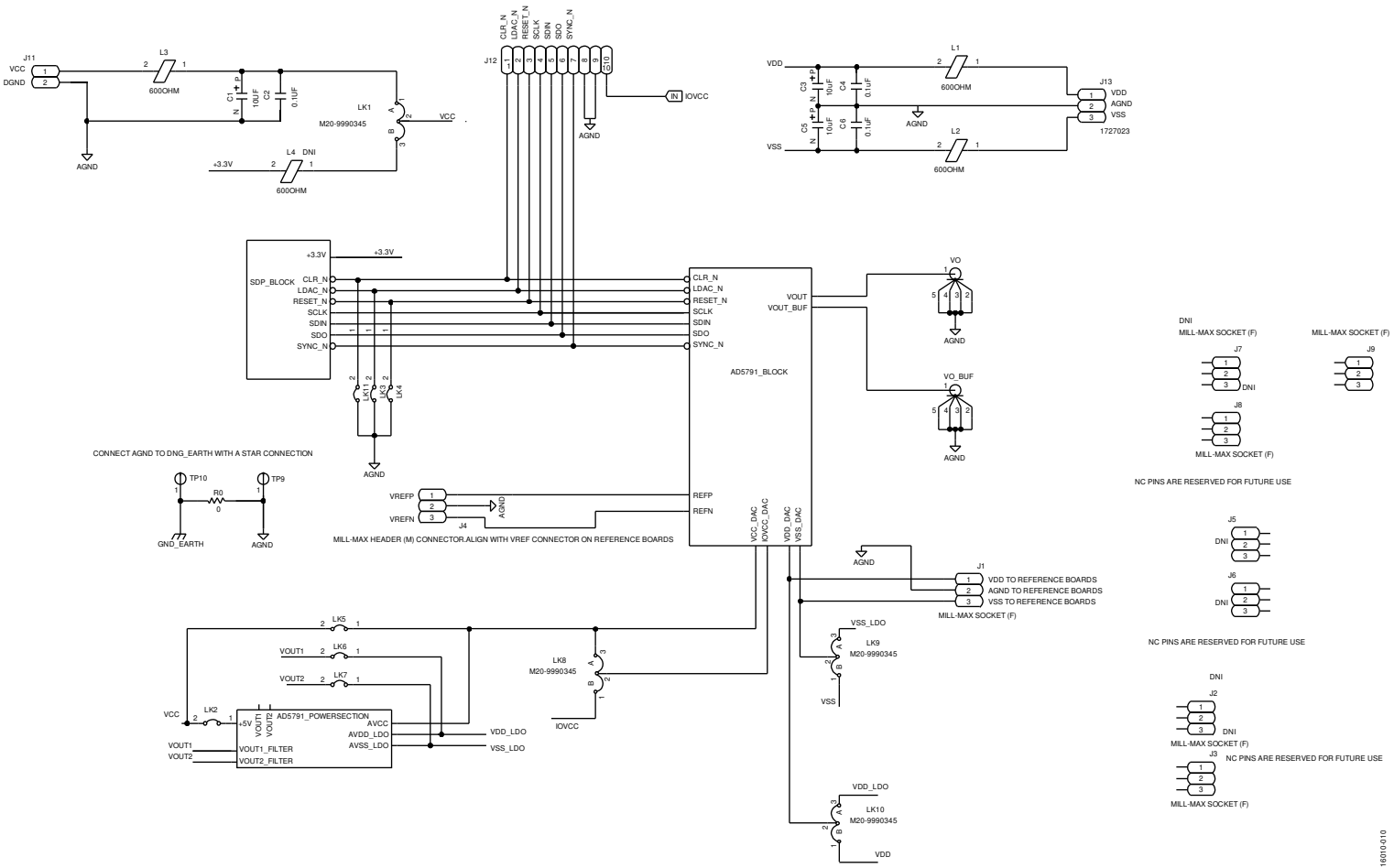
Figure 12. Schematic of the Main AD5791 Circuitry
