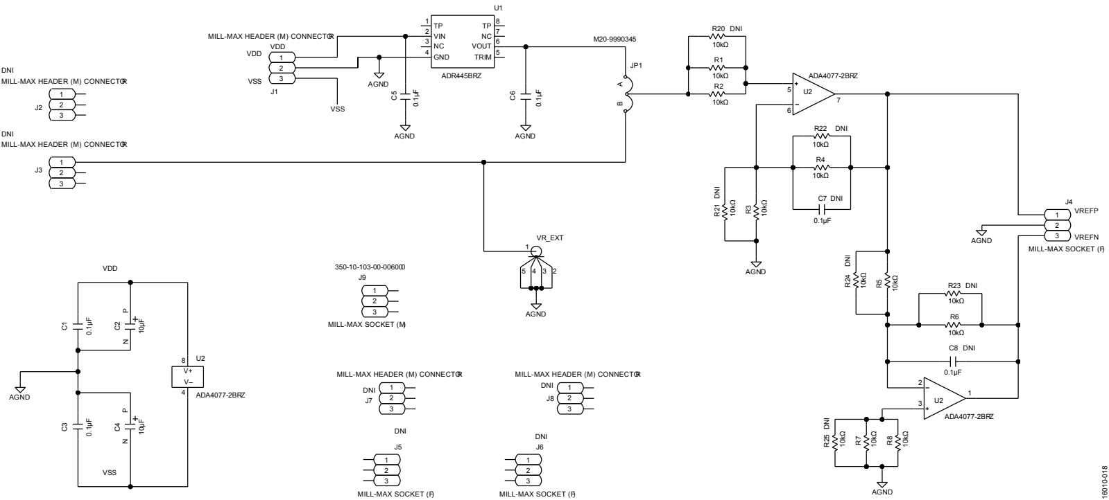
Figure 20. Schematic of the EV-ADR445-REFZ
