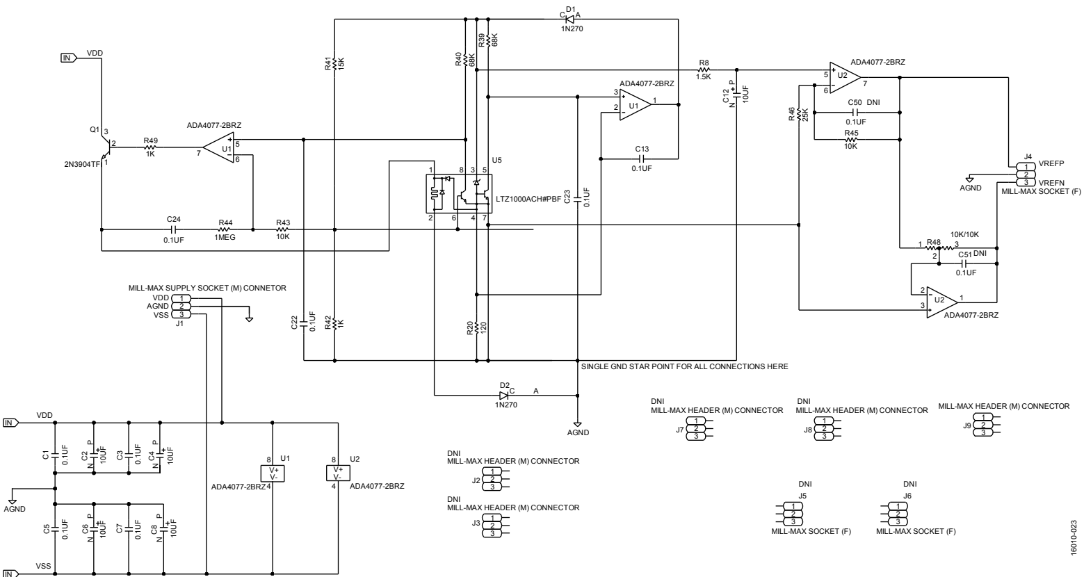
Figure 24. Schematic of the EV-LTZ1000-REFZ
