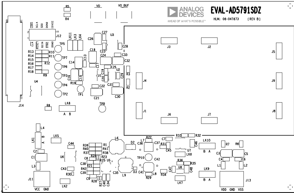
Figure 17. Component Placement Schematic
