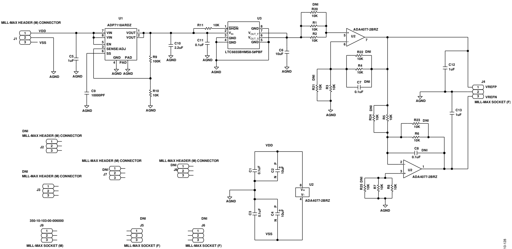
Figure 28. Schematic of the EV-LT6655-REFZ
