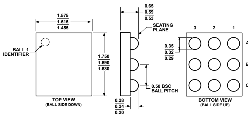
Figure 27. 9-Ball Wafer Level Chip Scale Package [WLCSP] (CB-9-1)
