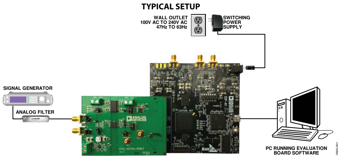
Figure 1. Typical Setup ( EVAL-AD7402-8FMCZ on Left and EVAL-SDP-CH1Z on Right)
