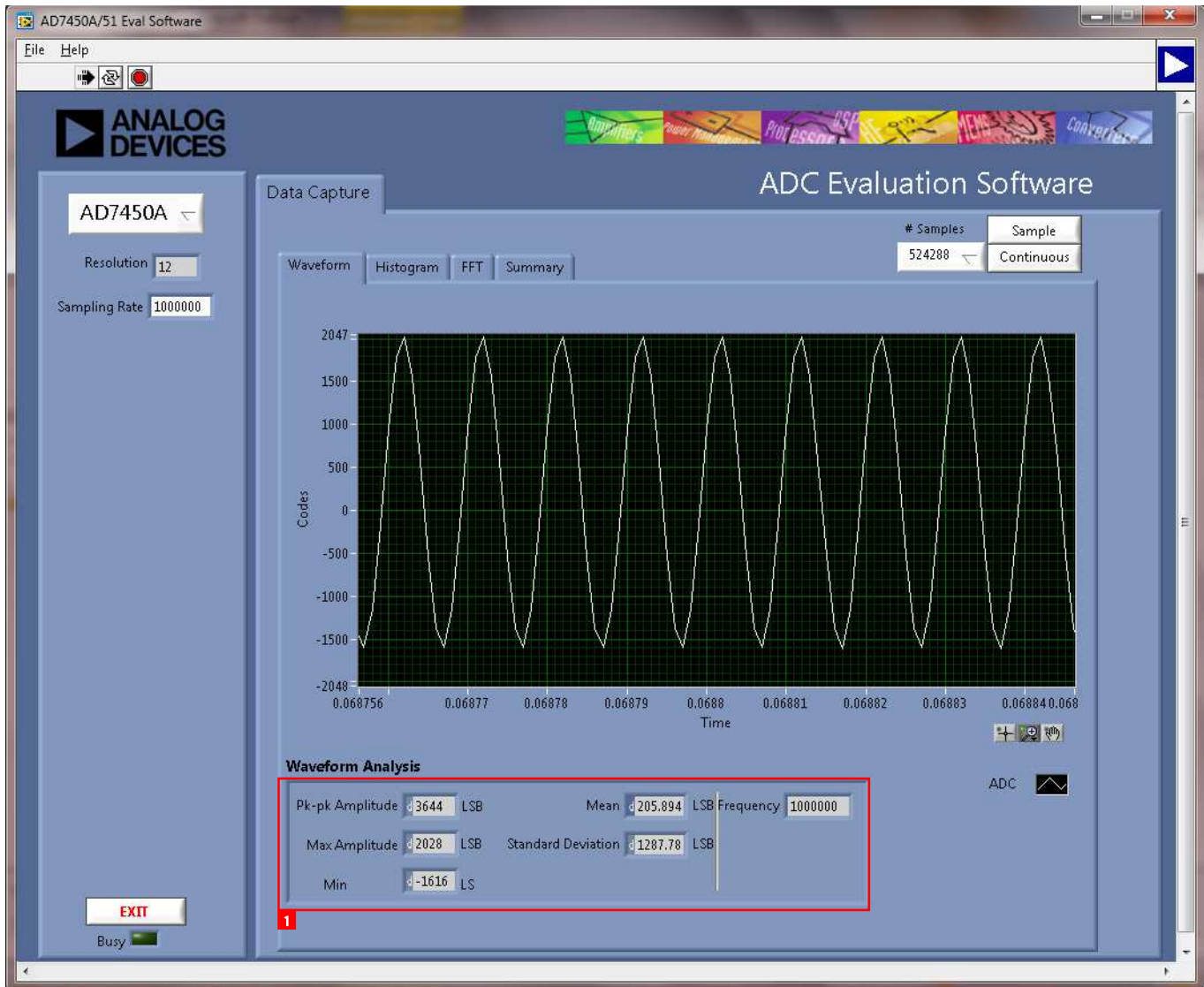
Figure 18. Waveform Tab
