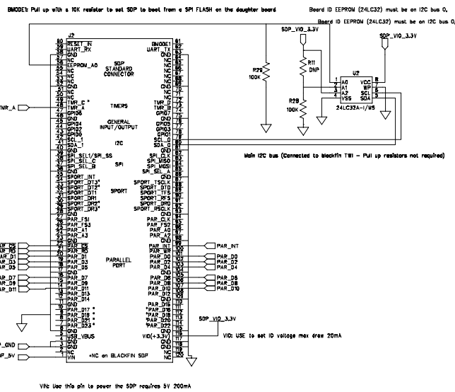
Figure 27. Schematic Page 5
